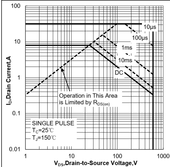
Figure 1a Safe Operating Area (TO-220/TO-251/TO-252)
