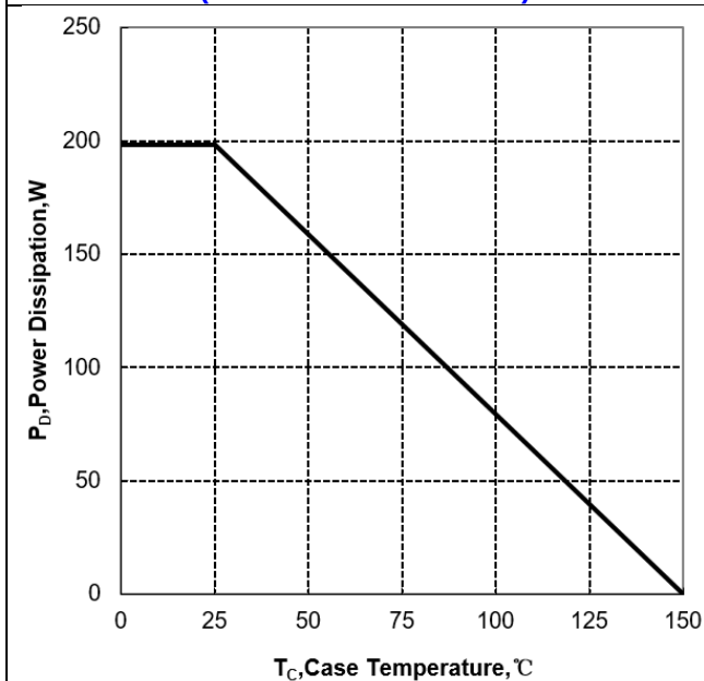
Figure 2a Power Dissipation (TO-220/TO-251/TO-252)
