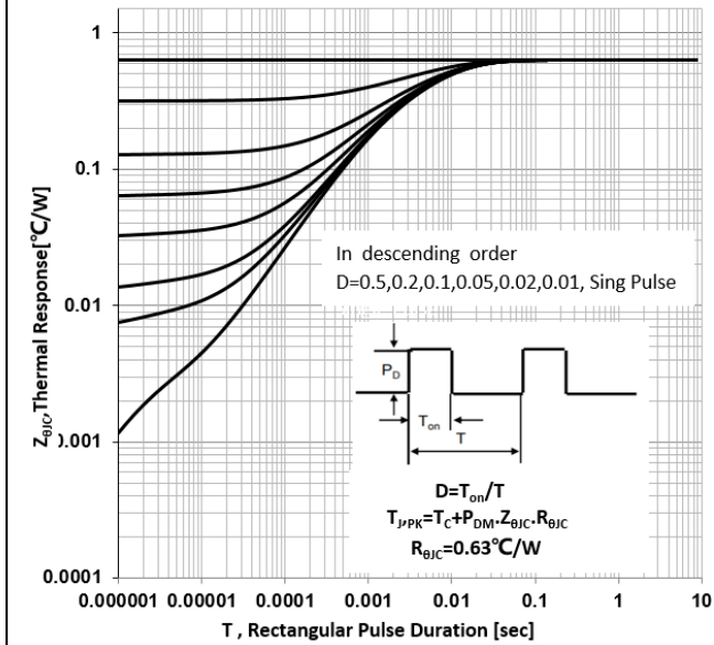
Figure 3a Max Thermal Impedance (TO-220/TO-251/TO-252)
